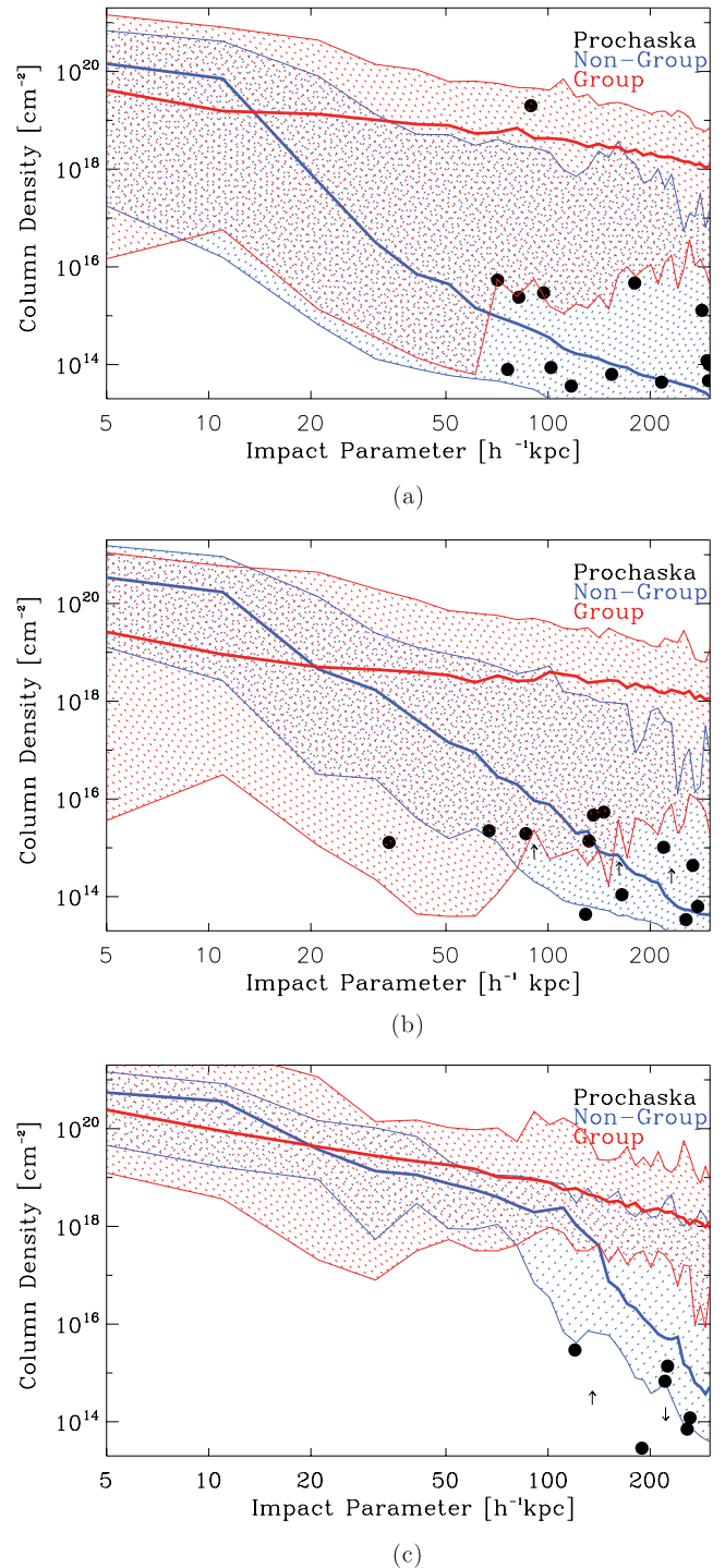
Figure 1. The solid lines represent the median of the stacked mean H I column densities as a function of impact parameter for galaxies in the stellar mass ranges (a) 10^9 – 10^{10} h^{-1} M_{\odot} (b) 10^{10} – 10^{11} h^{-1} M_{\odot} (c) >10^{11} h^{-1} M_{\odot} . The black dots correspond to the observations of background QSO absorbers along the lines-of-sight to foreground (a) <0.1L^* (b) \sim 0.1 – 1L^* (c) \sim L^* galaxies, from Prochaska et al. (2011). Coloured regions include the 5th and 95th percentiles for each bin. In all mass ranges, the radial profiles of the group galaxies are noticeably extended when compared to the galaxies in a non-group environment while in general our results are consistent with the observations of Prochaska et al. (2011).
