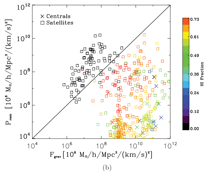
Figure 3. The axes represent the ram pressure exerted on each satellite (vertical axis) against the gravitational restoring force (horizontal axis) for both the non-group galaxies (crosses) and the group galaxies (squares). The colours from black to red indicate increasing H I ratios within the individual galaxies. We note, that black symbols (indicating very low H I ratios) lie predominantly above the diagonal where ram pressure exceeds the gravitational restoring force and are only satellite galaxies.
