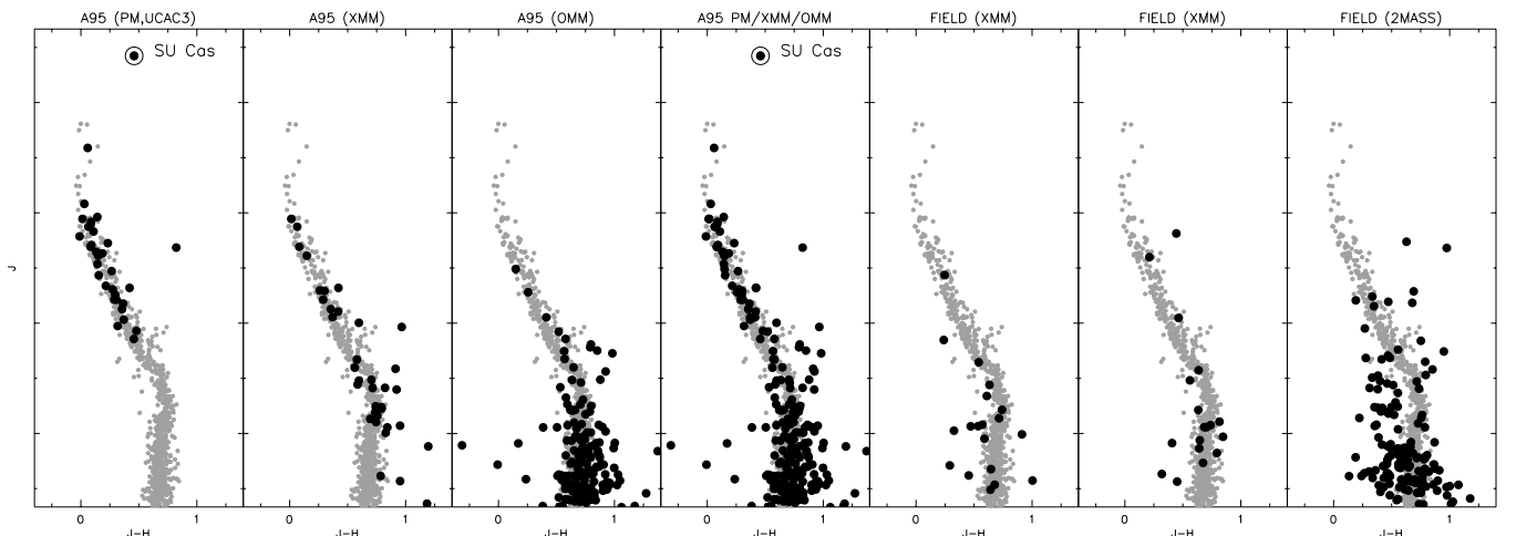
Figure 3. JH color-magnitude diagrams for stars exhibiting similar proper motions to SU Cas (PM, UCAC3), stars emitting X-rays ( XMM ), and OMM stars sampled r < 4' from the center of Alessi 95 (A95). Gray dots are calibration stars from Majaess et al. (2011b). Comparison fields sampled by XMM-Newton and 2MASS imply that the cluster (A95) distribution is not fortuitous.
