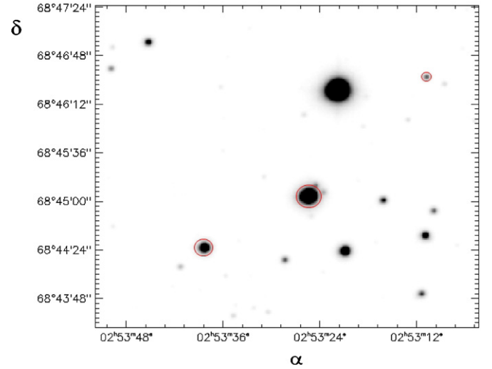
Figure 2. Finder chart (OMM J ) for three probable cluster members which are X-ray sources. The two brighter objects exhibit UCAC3 proper motions (e.g., \mu_\alpha : \mu_\delta = 0.8 \pm 1.0 : -8.2 \pm 0.8 \text{ mas yr}^{-1} ) matching that established for SU Cas ( \mu_\alpha : \mu_\delta = 1.0 \pm 0.7 : -8.6 \pm 0.8 \text{ mas yr}^{-1} ). The stars are probable cluster members based on X-ray, proper motion, and color-magnitude data (Figure 3). The finder chart represents a small portion of the observed field.
