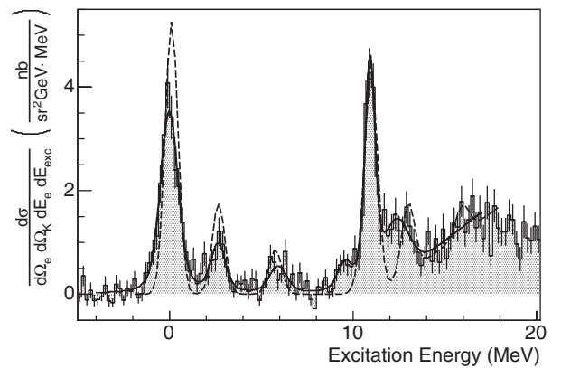
FIG. 3. The ^{12}_{\Lambda}\text{B} excitation-energy spectrum. The best fit (solid curve) and a theoretical prediction (dashed curve) are superimposed on the data. See text for details.
