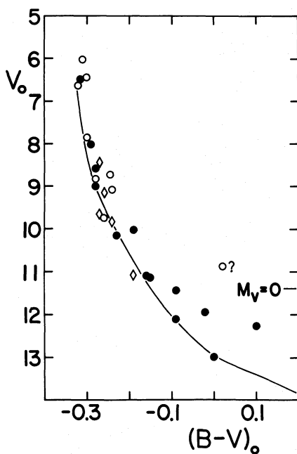
FIG. 4.—Reddening-free color-magnitude diagram for Stock 16 and its neighboring complex. Members of the cluster nucleus are indicated by filled circles, while open symbols denote nearby members of Cen OB1 (circles) and Cen R1 (diamonds).
