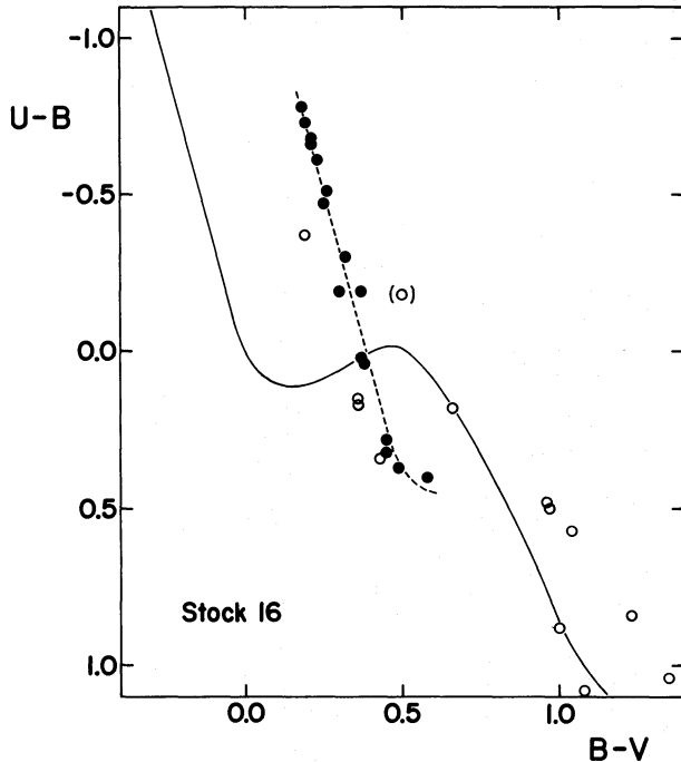
FIG. 3.—Color-color diagram for Stock 16, with likely cluster members denoted by filled circles. The dashed line represents the location of the intrinsic relation for main-sequence stars (solid line) reddened by E_{B-V} = 0.49 .
