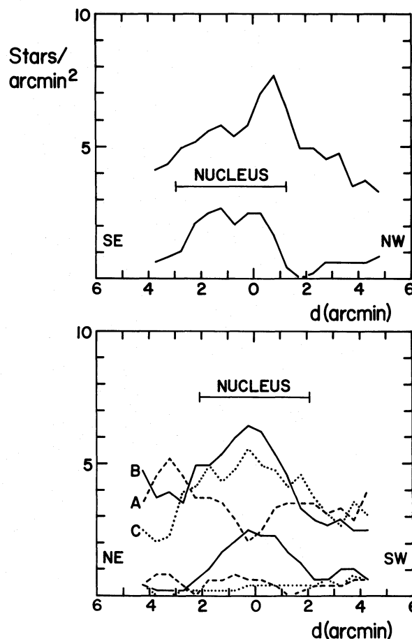
FIG. 5.—Strip counts for Stock 16 as described in the text. The upper relation in each section represents star densities above B \approx 18 , while the lower relation is for a limit of B \approx 15 . The three relations in the lower section are for strips 3' southeast of the cluster center (A), through the cluster center (B), and 3' northwest of the cluster center (C).
