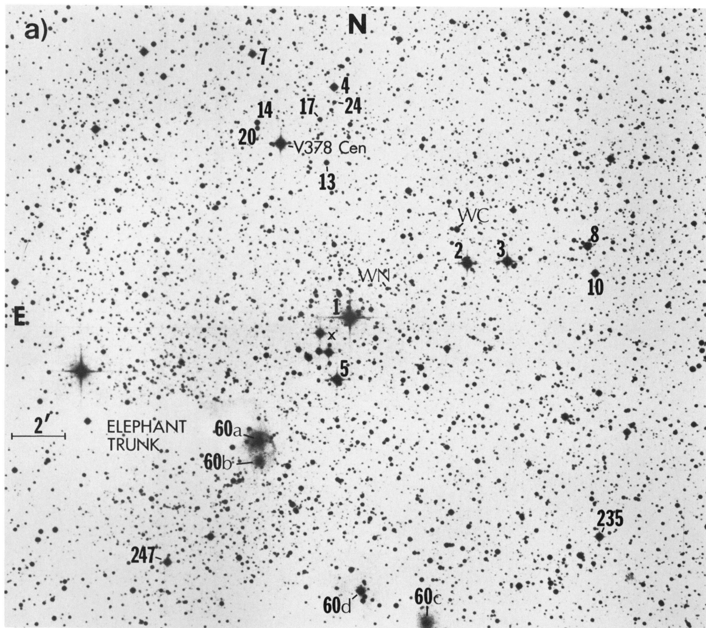
FIG. 2.—Identification chart for (a) the Stock 16 region, and (b) the cluster nuclear region as reproduced from the ESO B Survey plate (copyright European Southern Observatory ). Stars 1 to 33 are from Table 1, 60a, b, c, and d are from van den Bergh and Herbst 1975, and 235 and 247 are from Lyngå 1970a. The two W-R stars in the region are identified as WC (MR 44) and WN (MR 45), and X denotes the location of the cluster center found from star counts.
