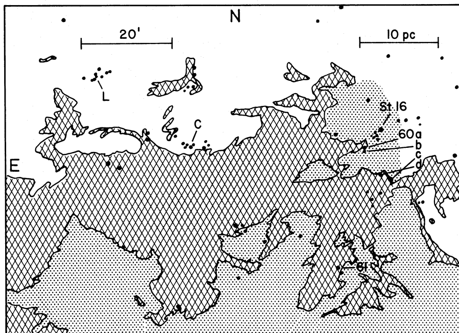
FIG. 1.—Schematic illustration of the Stock 16 region showing the prominent dust concentrations ( cross-hatching ) and emission nebulosity ( dots ). Symbols denote the stars in Cen R1 (60a, b, c, d, and 61), Stock 16 (St 16), and the star chain (C) and anonymous cluster (L) discussed in § VI.
