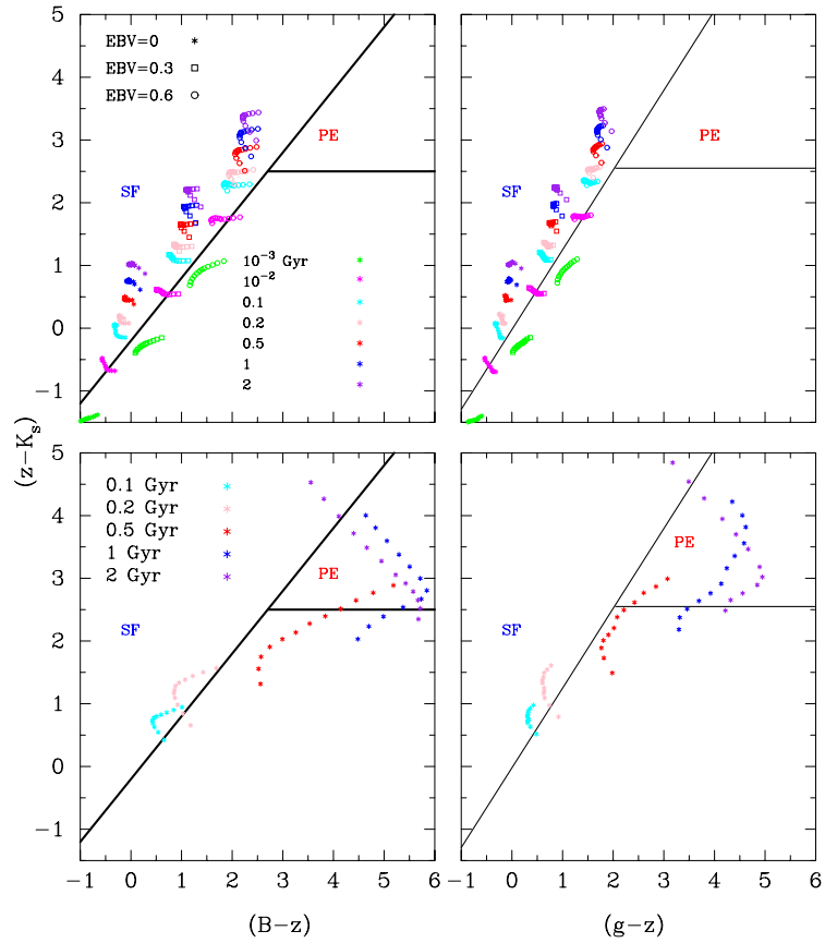
Figure 1.1: Two pairs of colour-colour diagrams, one on the left for BzK Selection and the one on the right for gzK Selection. Each set of data points is model galaxy on the colour-colour diagram, over a range of redshifts between 1.4 \leq z \leq 2.5 . The colour of the data points correspond to the age of the model galaxies, the shape of the data points correspond to variations in model extinction. (Arcila-Osejo and Sawicki (2013))
