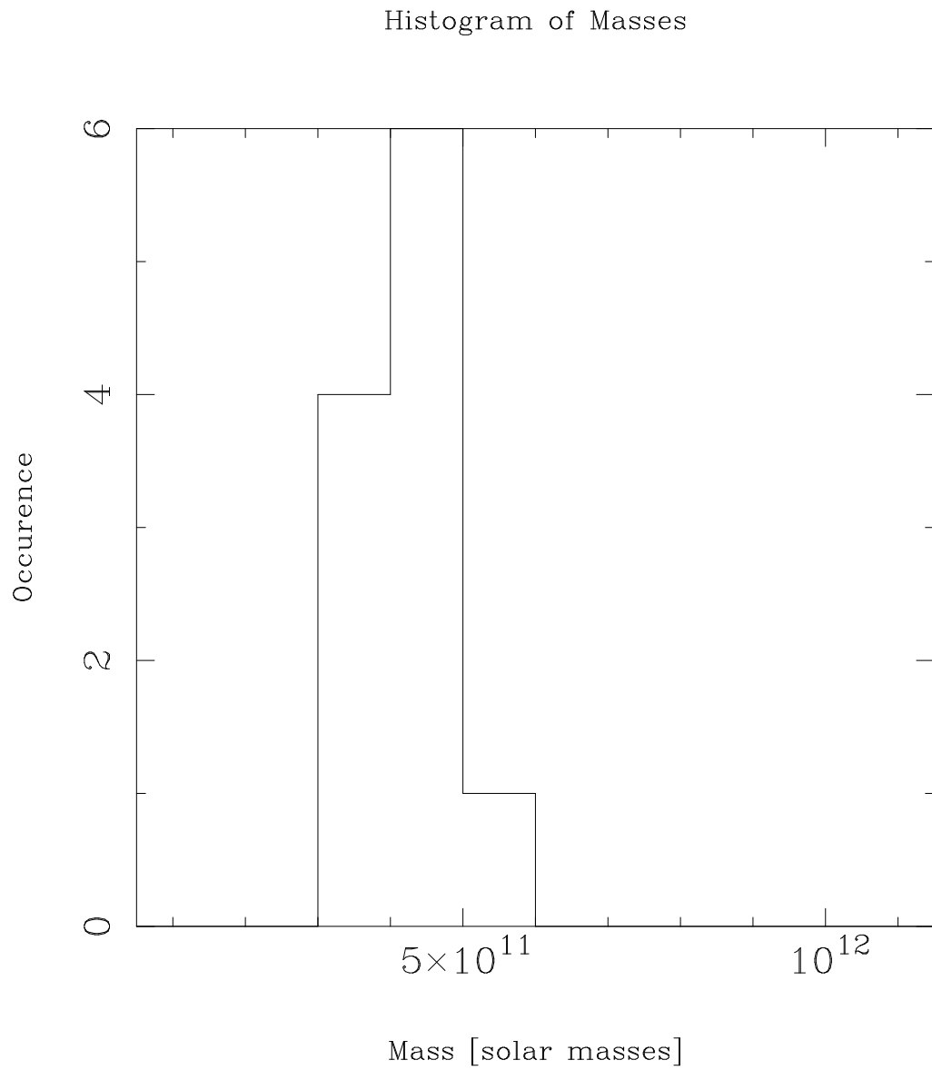
Figure 3.4: Histogram of Masses
