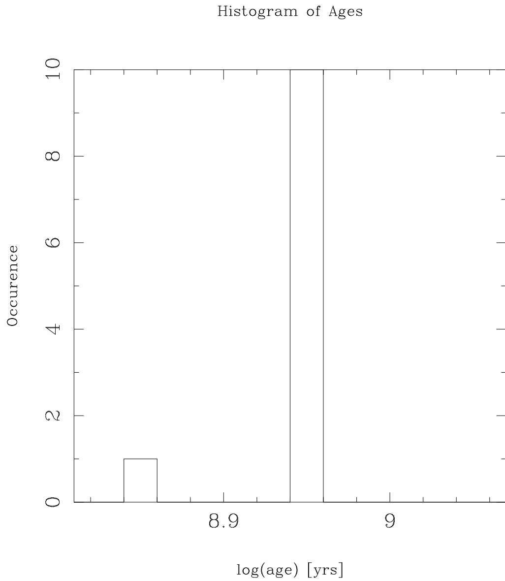
Figure 3.6: Histogram of Galaxy Ages
