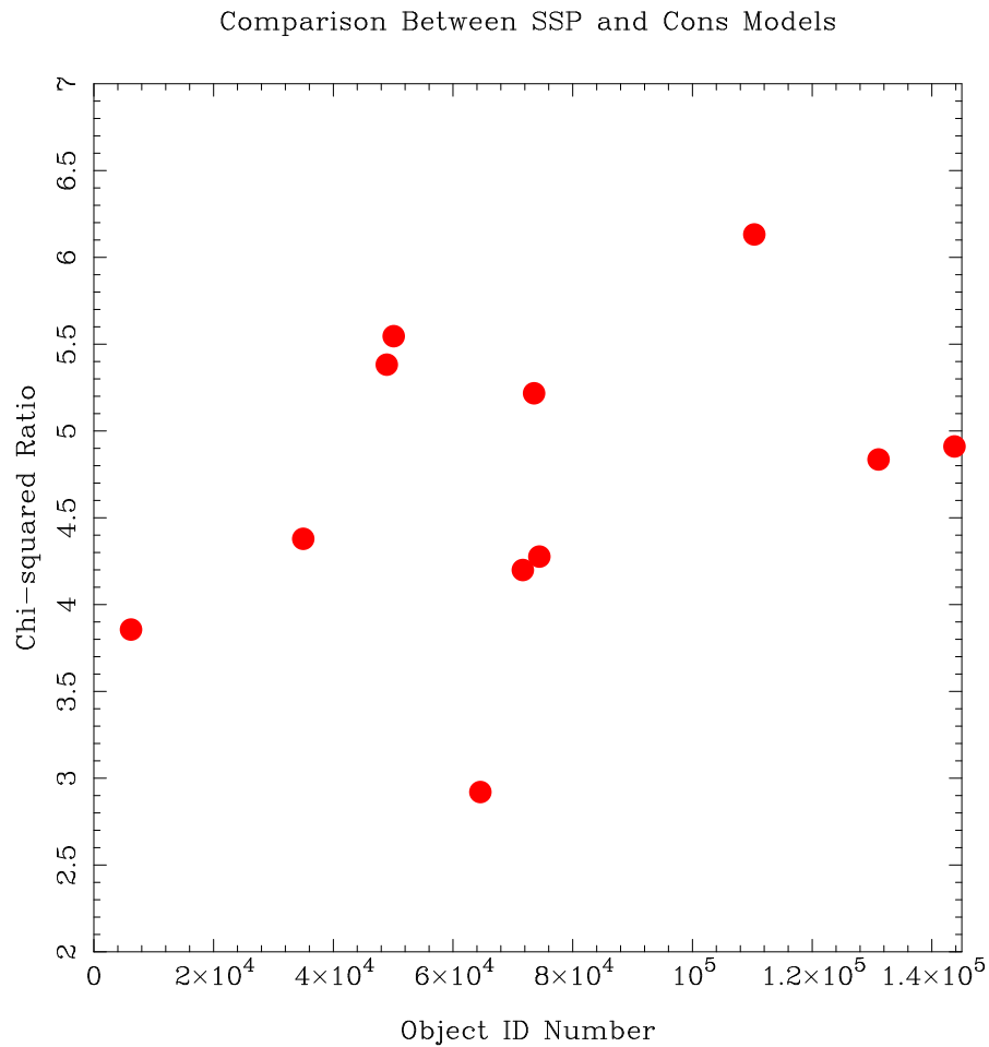
Figure 3.3: Comparison of SSP and Cons Model. Points shown are the ratio of \frac{\chi_{Cons}^2}{\chi_{SSP}^2} for each object. If the two models resulted in identical fits, the points would form a line at \frac{\chi_{Cons}^2}{\chi_{SSP}^2} = 1 . Since the points are above this line of unity, the \chi^2 values for the Cons model are greater than the \chi^2 values for the SSP model.
