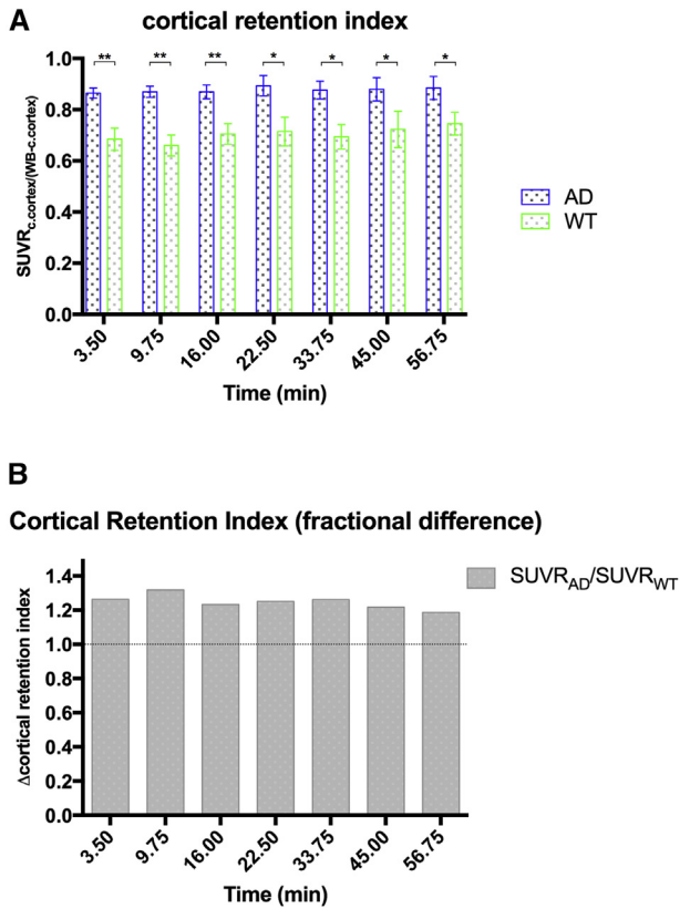
Fig. 6. A) N -methylpiperidin-4-yl 4- 123 Iiodobenzoate retention indices for 5XFAD (blue) and WT (green) mice. Mean \pm SEM. (A) Cortical retention index (SUVr cortex /(whole brain-cortex)); cortical retention normalized to rest-of-brain) was 18%–31% greater in 5XFAD brains versus WT over the 60-minute imaging window. ***Denote statistically significant differences ( P < .05 , P < .01 , respectively). (B) Fractional difference in cortical retention index between 5XFAD and WT indicating between 1.18–1.31X greater retention in the cerebral cortex of 5XFAD mice compared to WT. Abbreviations: AD, Alzheimer's disease; SEM, standard error of the mean; SUVr, relative standardized uptake value; WT, wild-type; 5XFAD, B6SJL-Tg(APP S SwFLon, PSEN1 M146L L286V) 6799Vas/Mmjax mouse strain.
