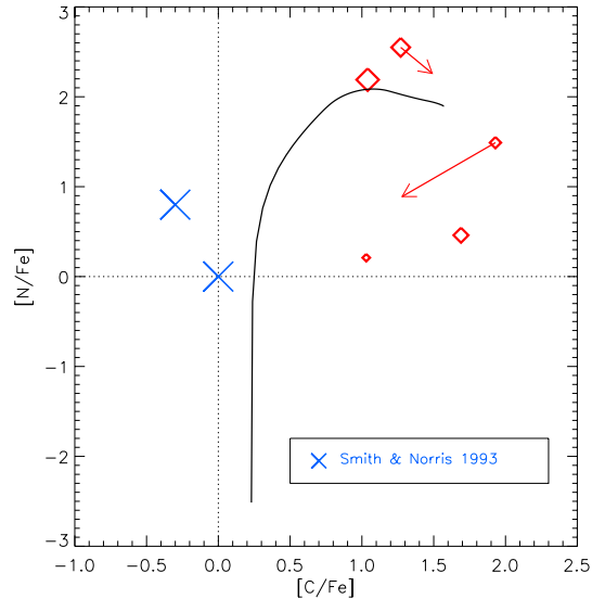
Figure 3. Predicted evolution of [\text{N/Fe}] with [\text{C/Fe}] (solid line). Symbols have the same meaning as in Fig. 1 except that crosses denote data from Smith & Norris (1993).
