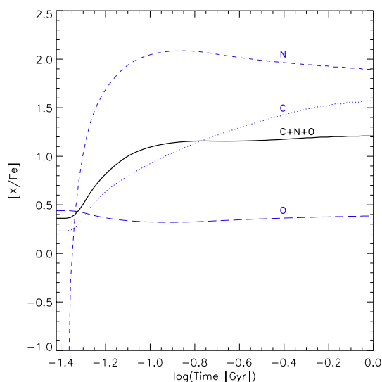
Figure 4. Temporal evolution of [C/Fe] (dotted line), [N/Fe] (short dashed line), [O/Fe] (long dashed line) and [C+N+O/Fe] (solid line). In contrast to observations in NGC 6752 and other globular clusters, C+N+O abundance is predicted to vary by an order of magnitude if AGB stars are responsible for the Na and Al enhancement.
