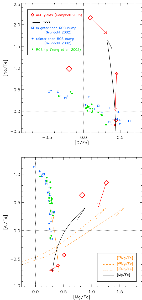
Figure 1. Predicted trend of [\text{Na}/\text{Fe}] versus [\text{O}/\text{Fe}] (a) and [\text{Al}/\text{Fe}] versus [\text{Mg}/\text{Fe}] (b) (thick curve) shown against observational data from Grundahl et al. (2002) (squares and pluses) and Yong et al. (2003) (circles). Data from Yong et al. were shifted on to the Grundahl et al. scale. Diamonds correspond to the 1.25, 2.5, 3.5, 5.0 and 6.5 M_{\odot} stellar models of Campbell (in preparation), where the size of the symbol indicates the stellar mass. Arrows indicate the effects of changing the mass-loss law for 2.5- and 5.0- M_{\odot} stars (see text for details). In the lower panel, the evolution of ^{24}\text{Mg}/\text{Fe} , ^{25}\text{Mg}/\text{Fe} and ^{26}\text{Mg}/\text{Fe} are shown by dotted, dashed, and dot-dashed lines, respectively.
