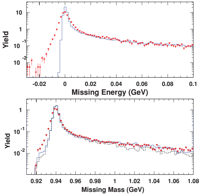
FIG. 14. (Color online) Comparison between data (triangles) and SIMC (histogram) for the missing-energy distribution for one of the {}^1\text{H}(e, e'p) kinematics (top) and for the missing-mass distribution for a representative {}^1\text{H}(e, e'\pi^+)n case (bottom). The solid histogram includes radiative effects and pions that pass through the HMS collimator. The latter events produce an additional contribution in the region M_m = 1.025\text{--}1.07 GeV. The dashed histogram represents simulated events without the effect of collimator punch-through.
