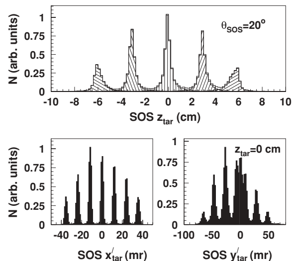
FIG. 9. SOS quintar and sieve-slit reconstruction. Top: reconstruction of the quintar z_{tar} coordinate. The distribution shown is the sum of the five individual targets (hashed). Bottom: reconstruction of the vertical (left) and horizontal (right) sieve-slit hole pattern.
