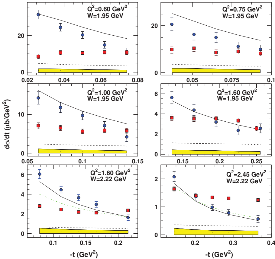
FIG. 17. (Color online) Separated cross sections, \sigma_L (circles) and \sigma_T (squares) at central values of Q^2 = 0.60, 0.75, 1.00, 1.60 \text{GeV}^2 ( W = 1.95 \text{GeV} ), and Q^2 = 1.60, 2.45 \text{GeV}^2 ( W = 2.22 \text{GeV} ). The values of \bar{W} and \bar{Q}^2 are different for each -t bin. The error bars for \sigma_L indicate the statistical and uncorrelated systematic uncertainties in both \epsilon and -t combined in quadrature. The error band denotes the correlated part of the systematic uncertainty by which all data points move collectively for \sigma_L . The error bars for \sigma_T represent the total uncertainty. The curves denote Regge calculations (VGL, [48,49]) for \sigma_L (solid line) and \sigma_T (dashed line) for \Lambda_\pi^2 = 0.462 \text{GeV}^2 and \Lambda_\rho^2 = 1.5 \text{GeV}^2 . Also shown is a calculation for \sigma_L (dashed-dotted line) using a generalized parton distribution (GPD) model [50] including power corrections.
