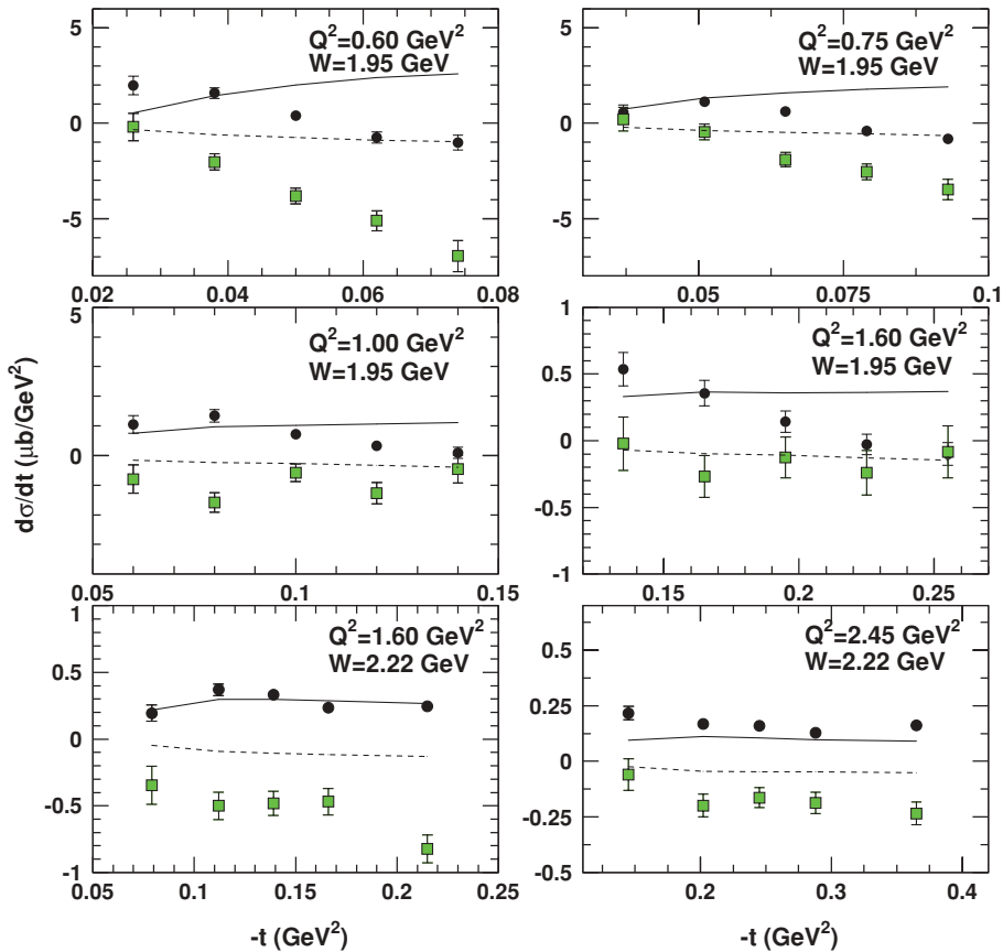
FIG. 18. (Color online) Interference terms, \sigma_{LT} (circles) and \sigma_{TT} (squares) at central values of Q^2 = 0.60, 0.75, 1.00, 1.60 \text{GeV}^2 ( W = 1.95 \text{GeV} ), and Q^2 = 1.60, 2.45 \text{GeV}^2 ( W = 2.22 \text{GeV} ). The curves denote Regge calculations (VGL [48,49]) for \sigma_{LT} (solid line) and \sigma_{TT} (dashed line) with \Lambda_\pi^2 = 0.462 \text{GeV}^2 and \Lambda_\rho^2 = 1.5 \text{GeV}^2 .
