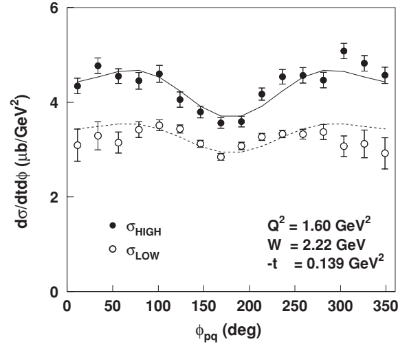
FIG. 16. Representative plot of the experimental cross sections, \frac{d^2\sigma}{dt d\phi} as a function of the azimuthal angle \phi_\pi at Q^2 = 1.60 ( \text{GeV}^2 ) for high and low \epsilon . The curves represent the fit of the measured values of the cross section to Eq. (12).
