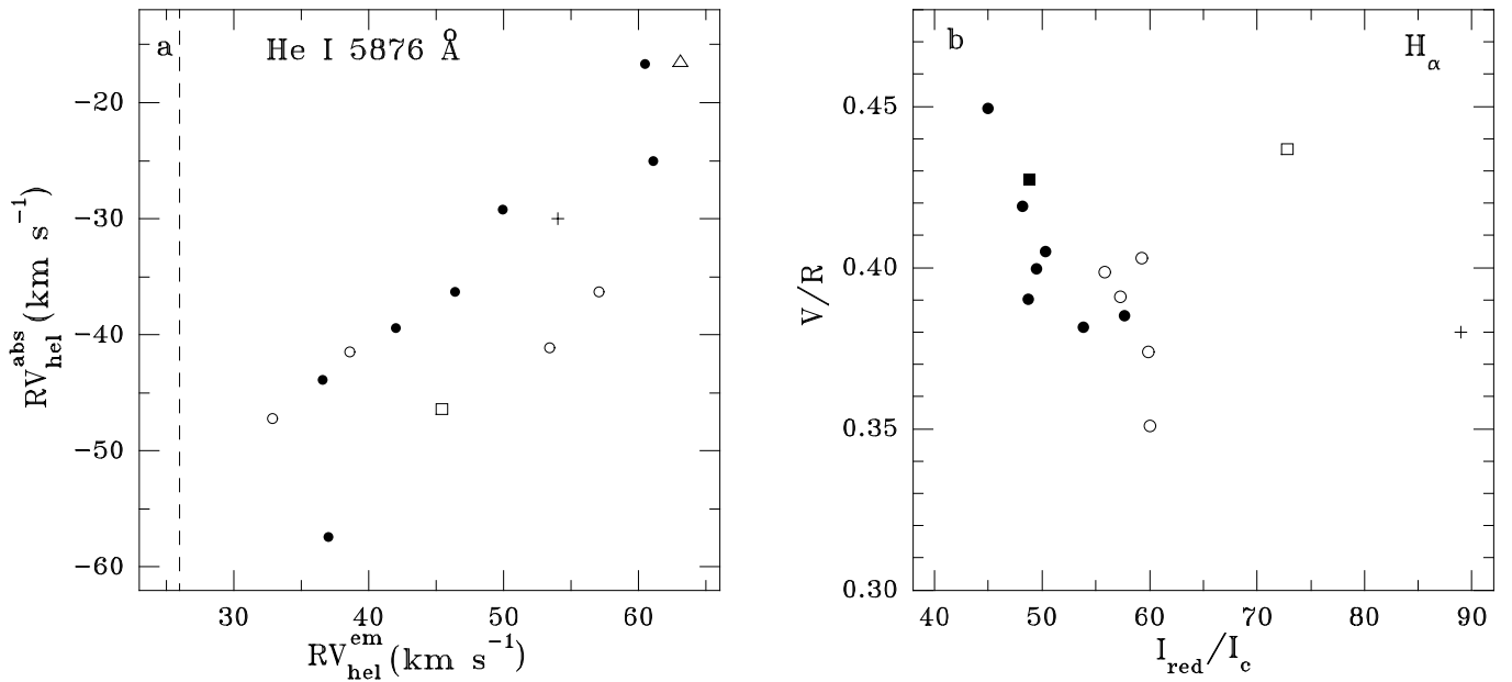
Fig. 5. Characteristics of emission lines in the spectrum of MWC 300. Panel a ) shows the relationship between the RV s of the absorption and emission component of the He I \lambda 5876 Å line. The vertical dashed line represents the mean position of the single-peaked emission lines (Fe II, Si II, etc.). Panel b ) shows the relationship between the peak intensity ratio and the strength of the red peak of the H\alpha line. Data from different observatories: filled circles – OHP, open circles – Leoncito, open square – McDonald, filled square – CFHT, open triangle – ESO, crosses – data from Zickgraf (2003). The RV s are heliocentric, and the intensities are in continuum units.
