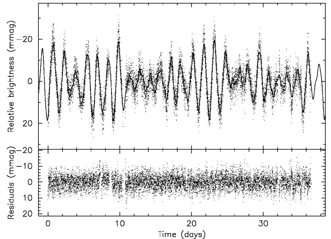
FIG. 1.— Top : Observed light curve of HD 163830 ( dots ) compared with the final fit given in eq. (1) ( solid line ). Bottom : Residuals after subtraction of the final fit.
