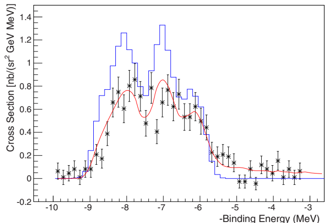
FIG. 3. (Color online) The 9 Li differential cross section as a function of the binding energy. Experimental points vs Monte Carlo results (red curve) and vs Monte Carlo results with radiative effects turned off (blue histogram).
