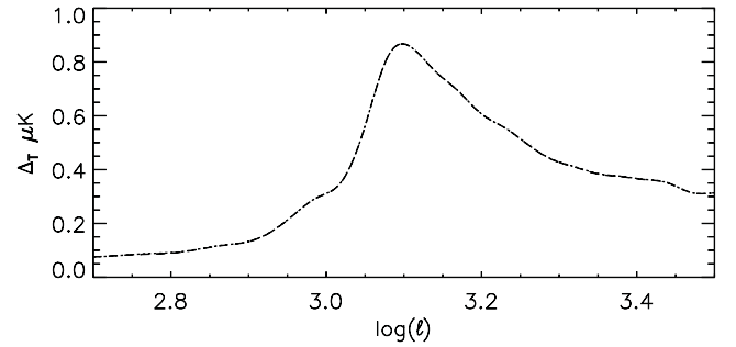
Figure 4. \Delta_T power spectrum in terms of \log(\ell) for different final RS integration/simulation redshifts. Dotted (dashed) line corresponds to a reference RSS which has been stopped at z_f = 0.5 ( z_f = 0.2 ). The curves are indistinguishable.
