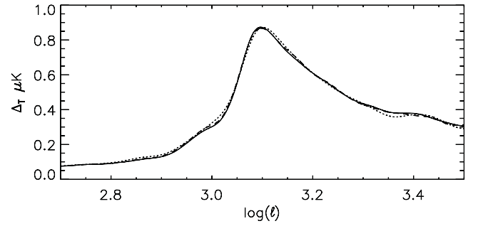
Figure 3. Quantity \Delta_T as a function of \log(\ell) for varying numbers of averaged RSSs. The averaged power \Delta_T obtained with three (dotted line), six (dashed), and nine (solid) reference RSSs are shown.
