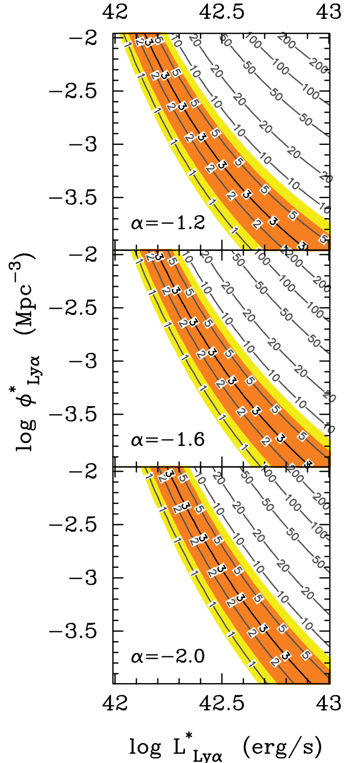
FIG. 10.—Mean number of LAEs detected in our experiment for different values of the intrinsic luminosity function parameters. From top to bottom, the panels show faint-end slope \alpha = -1.2 , -1.6 , and -2.0 . The y -axis is the normalization of the luminosity function, \phi_* . The x -axis is the characteristic luminosity L_* . The orange and yellow shading marks the 84.1% and 95% confidence regions, respectively, for detecting three LAEs.
