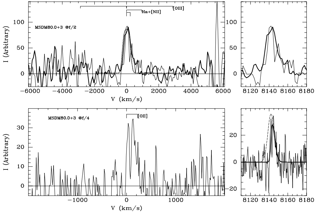
FIG. 4.—LAE MSDM 80+3. Velocity scale, tick marks, and arc line are as in Fig. 3. Top : IMACS f/2 spectra from 2005 May ( thin gray line ) and 2007 February ( thick black line ). Bottom left : IMACS f/4 spectrum. Bottom right : IMACS f/4 spectrum and fit. The model is a Gaussian ( 330 \text{ km s}^{-1} FWHM) with flux blueward of the peak set to zero and a 150 \text{ km s}^{-1} wide Gaussian 330 \text{ km s}^{-1} redward of the first. These components were convolved with another Gaussian representing instrumental broadening ( 150 \text{ km s}^{-1} ). [See the electronic edition of the Journal for a color version of this figure.]
