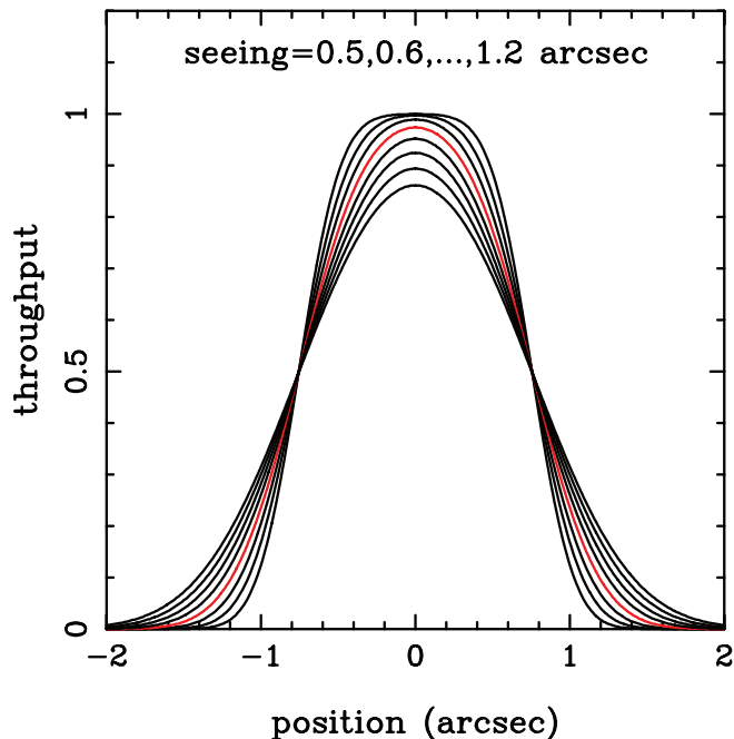
FIG. 9.— Attenuation of flux vs. offset from center of 1.5'' wide slit. Slit losses are shown for seeing-convolved sources with Gaussian surface brightness profiles of FWHM 0.5''\text{--}1.2'' in steps of 0.1'' . The red line represents the worst effective image quality in our survey.
