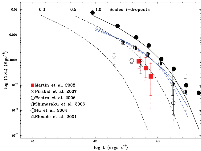
FIG. 12.—Comparison of cumulative number density of z = 5.7 LAEs and i -dropouts. Blue lines show the fitted luminosity distribution of LAEs from Shimasaku et al. (2006) with faint-end slope \alpha = -2.0 , -1.5 (solid line), and -1.0 . Black lines show the adopted fit to the distribution of i -dropouts from Bouwens et al. (2007); for purposes of illustration, we adopt constant \text{Ly}\alpha escape fractions of f_{\text{Ly}\alpha} = 1.0 , 0.5 , and 0.3 . The dashed black line illustrates the magnitude of some systematic uncertainties in the luminosity distribution fit, and filled circles show the i -dropout counts, converted to \text{Ly}\alpha luminosity using f_{\text{Ly}\alpha} = 1.0 .
