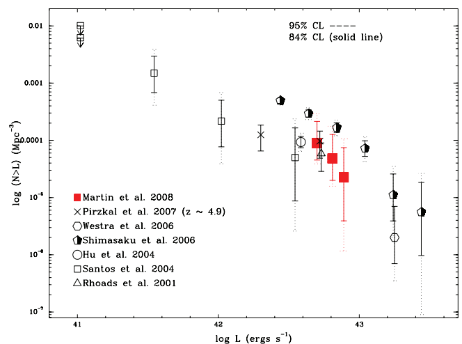
FIG. 11.—Cumulative number density of LAEs. Our best estimate is shown by the filled squares; the error bars are discussed in the note to Table 4. We compare number densities from the following narrowband imaging surveys: LALA 2001 ( triangle ), Hu et al. (2004; circle ), Westra et al. (2006; hexagon ), and Shimasaku et al. (2006; pentagon ). Spectroscopic results are shown from GRAPES (Pirzkal et al. 2007; cross ) and a program that positioned long slits along cluster caustics (Santos et al. 2004; open squares ).
