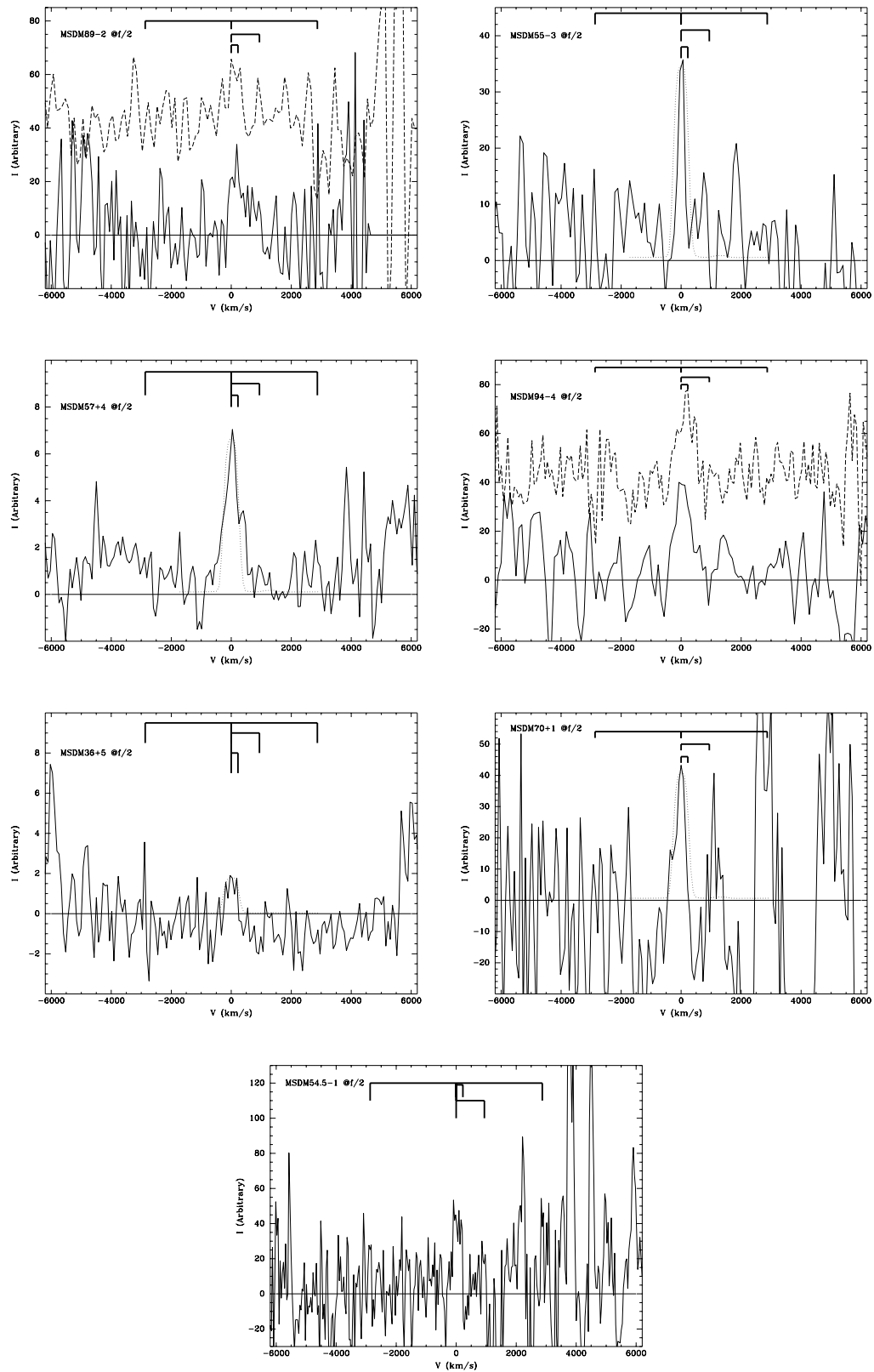
FIG. 7.—Low-resolution IMACS spectra of 15H field LAE candidates. The objects shown have a single line in the observed-frame 5000–9000 Å bandpass. This inset shows that no lines are seen at the spacing ( tick marks ) of the foreground contaminants [O II] \lambda\lambda 5007, 4959 or H \alpha +[N II] \lambda 6584. Comparison to the profile ( dotted line ) of a source that fills the slit shows that the lines are unresolved, and higher resolution spectroscopy is required to show line asymmetry and/or identify the [O II] \lambda\lambda 3726, 3729 doublet ( small ticks ).
