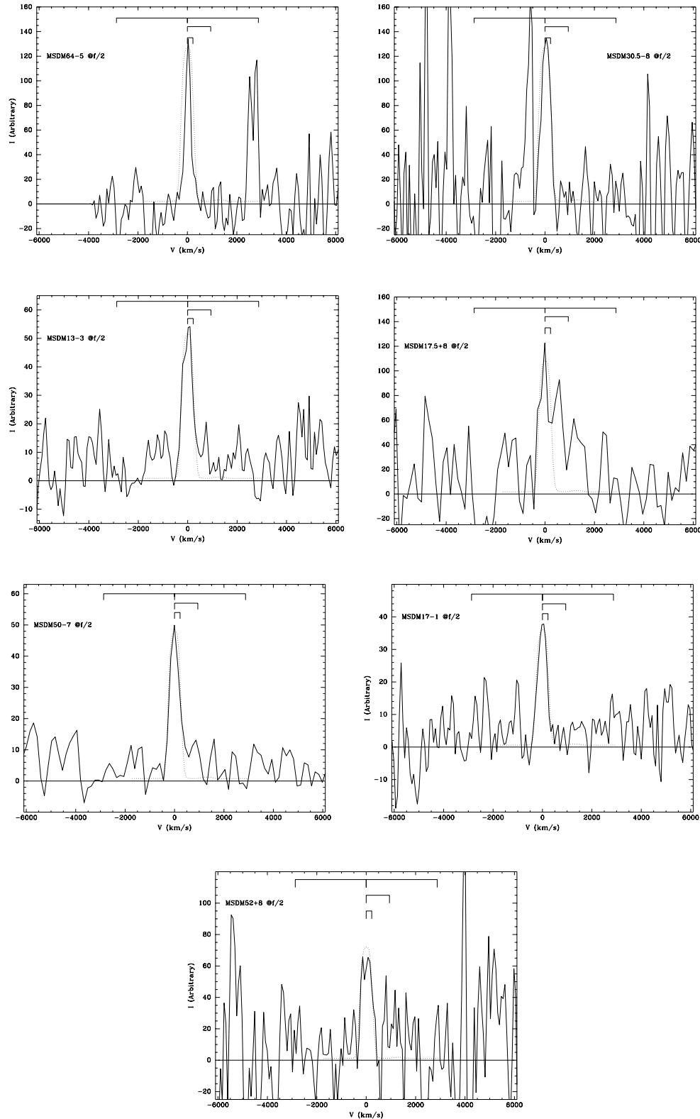
FIG. 6.—Low-resolution ( f/2 ) spectra of 10H field LAE candidates. The objects shown have a single line in the observed-frame 5000–9000 Å bandpass. This inset shows that no lines are seen at the spacing (tick marks) of the foreground contaminants [O III] \lambda\lambda 5007, 4959 or H\alpha + [N II] \lambda 6584 . Comparison to the profile (dotted line) of a source that fills the slit shows that the lines are unresolved, and higher resolution spectroscopy is required to show line asymmetry and/or identify the [O II] \lambda\lambda 3726, 3729 doublet (small ticks).
