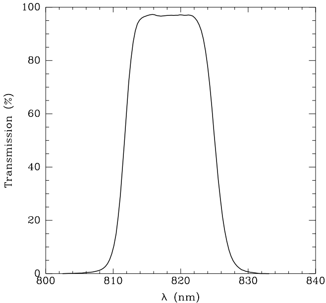
Fig. 1.—Transmission of the NB8190 filter.
