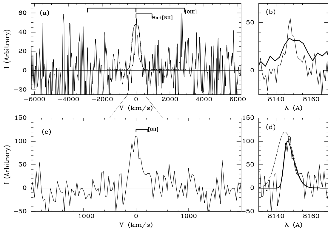
FIG. 3.—LAE MSDM 29.5+5. The zero point of the velocity scale is arbitrary, defined with zero at maximum intensity for convenience. Ticks mark the separations of lines that commonly appear in our spectra of foreground interlopers. (a) IMACS 200-1 f/2 spectrum taken in 2005 June. The line is narrow compared to the profile of a sky line, shown by the dotted line. (b) Spectrum from (a) on a wavelength scale. Also shown is an IMACS 150-1 f/2 spectrum taken in 2006 June (thick black line). (c) Higher resolution Keck LRIS spectrum. The line is asymmetric and skewed to the red. (d) Keck LRIS spectrum and fit. The model is a Gaussian ( 400 \text{ km s}^{-1} FWHM) with flux blueward of the peak set to zero and then convolved with another Gaussian representing instrumental broadening ( 110 \text{ km s}^{-1} ). [See the electronic edition of the Journal for a color version of this figure.]
