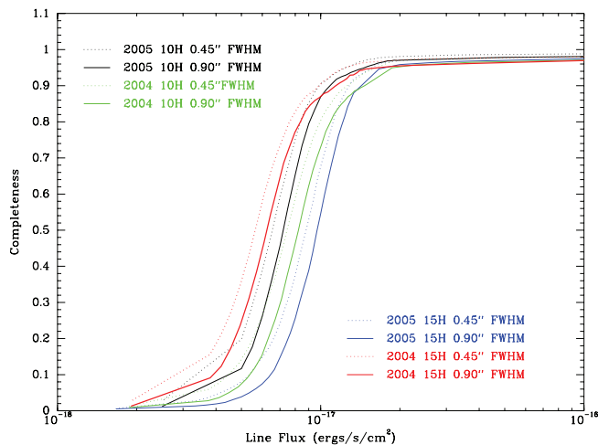
FIG. 8.— Completeness of emission-line surveys for two limiting source sizes. For the 2005 search in the 10H field, the line flux corresponding to 50% completeness is (6.6\text{--}7.2) \times 10^{-18} ergs \text{s}^{-1} \text{cm}^{-2} for sources between 0.45'' and 0.90'' FWHM.
