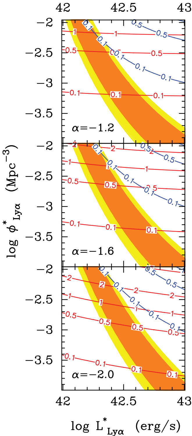
FIG. 13.—Total Ly \alpha luminosity density for the three values of the faint-end slope. Two lower limits are illustrated: (1) our survey detection limit of \log L = 42.57 \text{ erg s}^{-1} (blue contours), and (2) an extrapolation to \log L = 41.00 \text{ erg s}^{-1} (red contours), which corresponds to dwarf galaxies with \text{SFR} = 0.095 f_{\text{Ly}\alpha}^{-1} . The critical number of sources required to keep the IGM ionized is marked in units of the parameters C_6(1 - 0.1 f_{\text{Ly}\alpha,0.1}) f_{\text{Ly}\alpha,0.5} / f_{\text{Ly}\alpha,0.1} = 1.0 . With the lower limit in limit 1, it appears unlikely that enough galaxies have been discovered to keep the IGM ionized at z = 5.7 . It appears, however, from limit 2 that an extension of this population to lower luminosities, even with a shallow faint-end slope like \alpha = -1.2 , could easily produce the missing ionizing photons.
