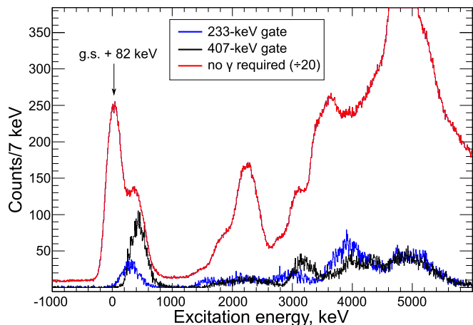
Fig. 2. (Colour online.) Excitation energy spectrum for states in ^{26}\text{Na} , reconstructed from the measured energy and angle of the protons from the d(^{25}\text{Na}, p) reaction. The spectrum for all events is shown (red), plus the results for coincidences with the known gamma-rays of 233 keV (blue) and 407 keV (black histogram) in ^{26}\text{Na} . The data are for proton laboratory angles backward of 90^\circ . A TRIFOIL requirement has been imposed in all cases (see text).
