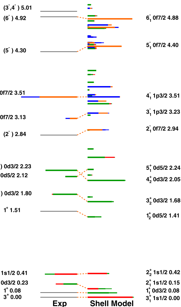
Fig. 5. (Colour online.) Level scheme of ^{26}\text{Na} as deduced from the present work compared to the results of shell model calculations employing the USD-A and WBP-M interactions (see text). The lengths of the coloured lines correspond to the spectroscopic factors as follows: red s -wave, blue p -wave, green d -wave, orange f -wave.
